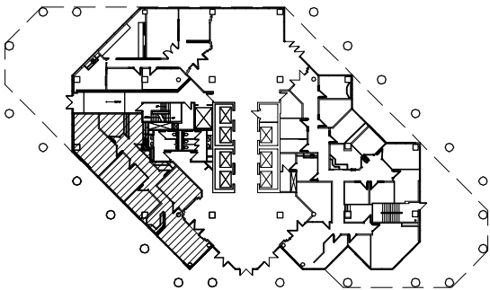
FIRST FLOOR KEY PLAN
